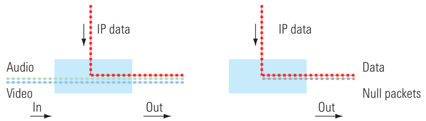
Left: R&S DIP010 with MPEG-2 input and output; right: R&S DIP010 with MPEG-2 output only
